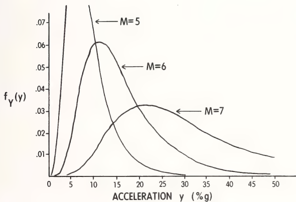
FIG. 4- DISTRIBUTION OF ACCELERATION, 3 PREDICTED EARTHQUAKES.
